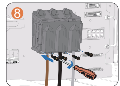
8 Secure the snap-fits and tighten the screws
