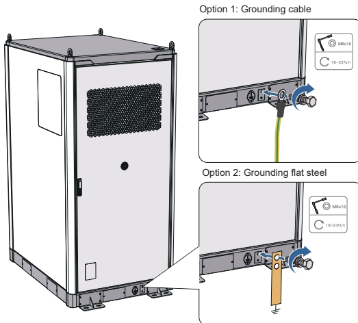
Option 1: Grounding cable
